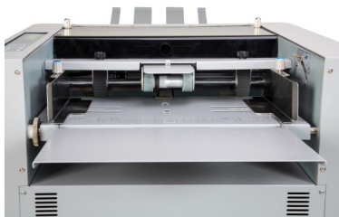
Wide access for SRA3 sheets: enabling a production of 24 business cards in one pass
