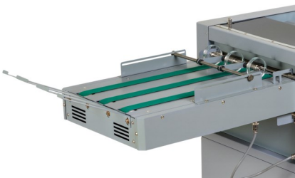
Standard 38 cm long conveyor allowing uninterrupted and lengthy production runs
