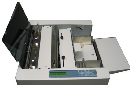
Special slot for optional scoring and perforating cassettes
